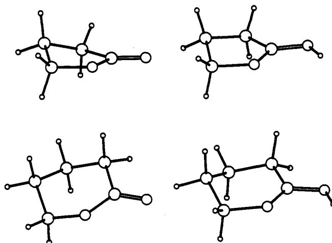
Figure 4. Structures of butyrolactone, valerolactone, and their protonated derivatives.
