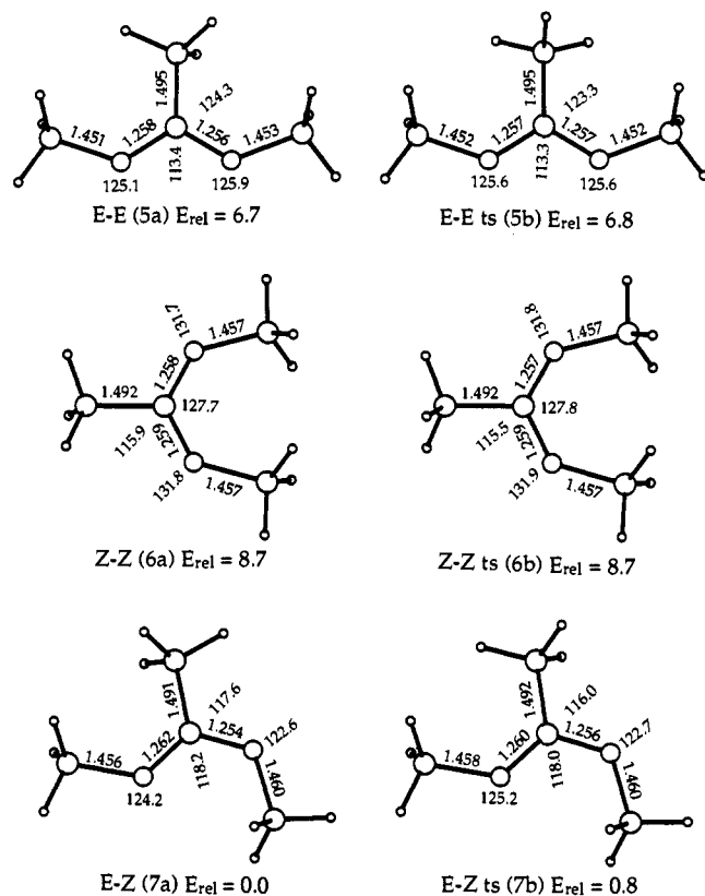
Figure 3. Structures of methylated methyl acetates. The ground-state structures are given to the left, and the transition states for methyl rotation are given to the right.
