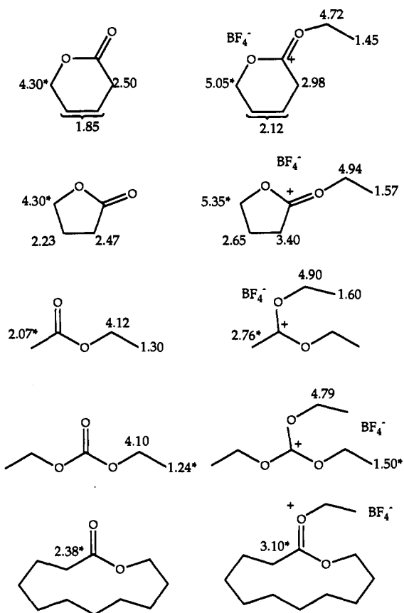
Figure 5. Chemical shifts for methylated esters and lactones. The bands used for determining the concentrations are marked with an asterisk.
