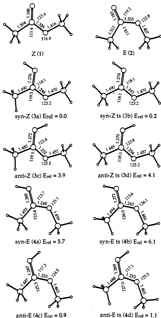
Figure 1. Structures of ( Z )- and ( E )-methyl acetates and their protonated forms. For the latter, the ground-state conformers are given at the left, and the corresponding transition states for methyl rotation are given at the right. Syn and anti refer to the orientation of the added proton with respect to the acetyl methyl group.
