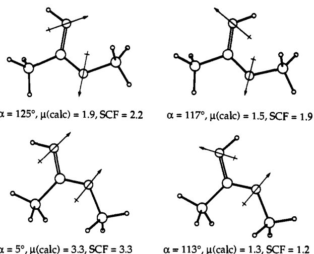
Figure 2. Orientation of the dipoles at oxygen for the protonated methyl acetates. The angle between the dipoles is given, along with an estimate of the dipole moment based on an oxygen dipole of 1.65 D. The SCF dipoles are those derived from the MO calculations.
